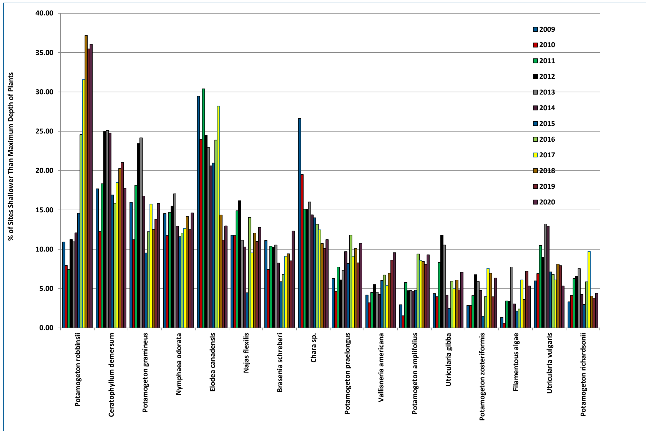
Figure 8-1 2009-2020 Beaver Dam Lake Frequency of Occurrence (% of Sites Shallower Than Maximum Depth of Plants)
