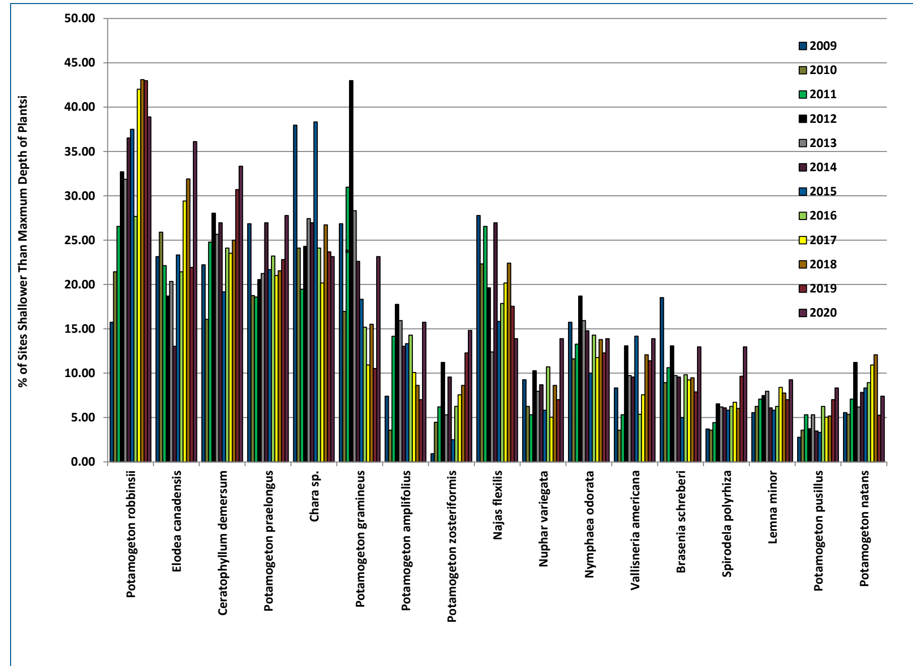
Figure 8-13 2009-2020 Rabbit Island Bay Frequency of Occurrence (% of Sites Shallower Than Maximum Depth of Plants)
