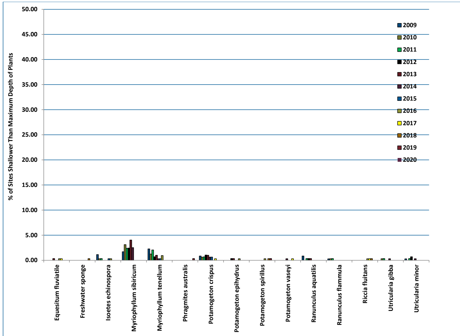
Figure 8-10 2009-2020 West Lake Frequency of Occurrence (% of Sites Shallower Than Maximum Depth of Plants)
