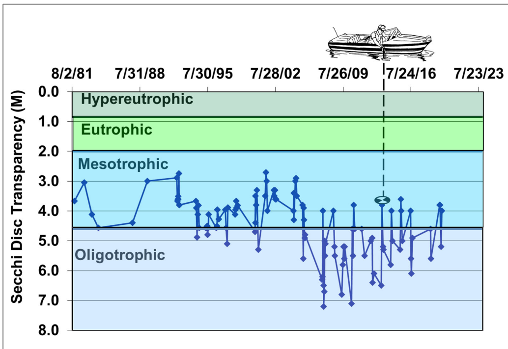
Figure 5-2 1981-2019 Beaver Dam Lake Secchi Disc Transparencies: West Lake (NE of Eagle Point)
