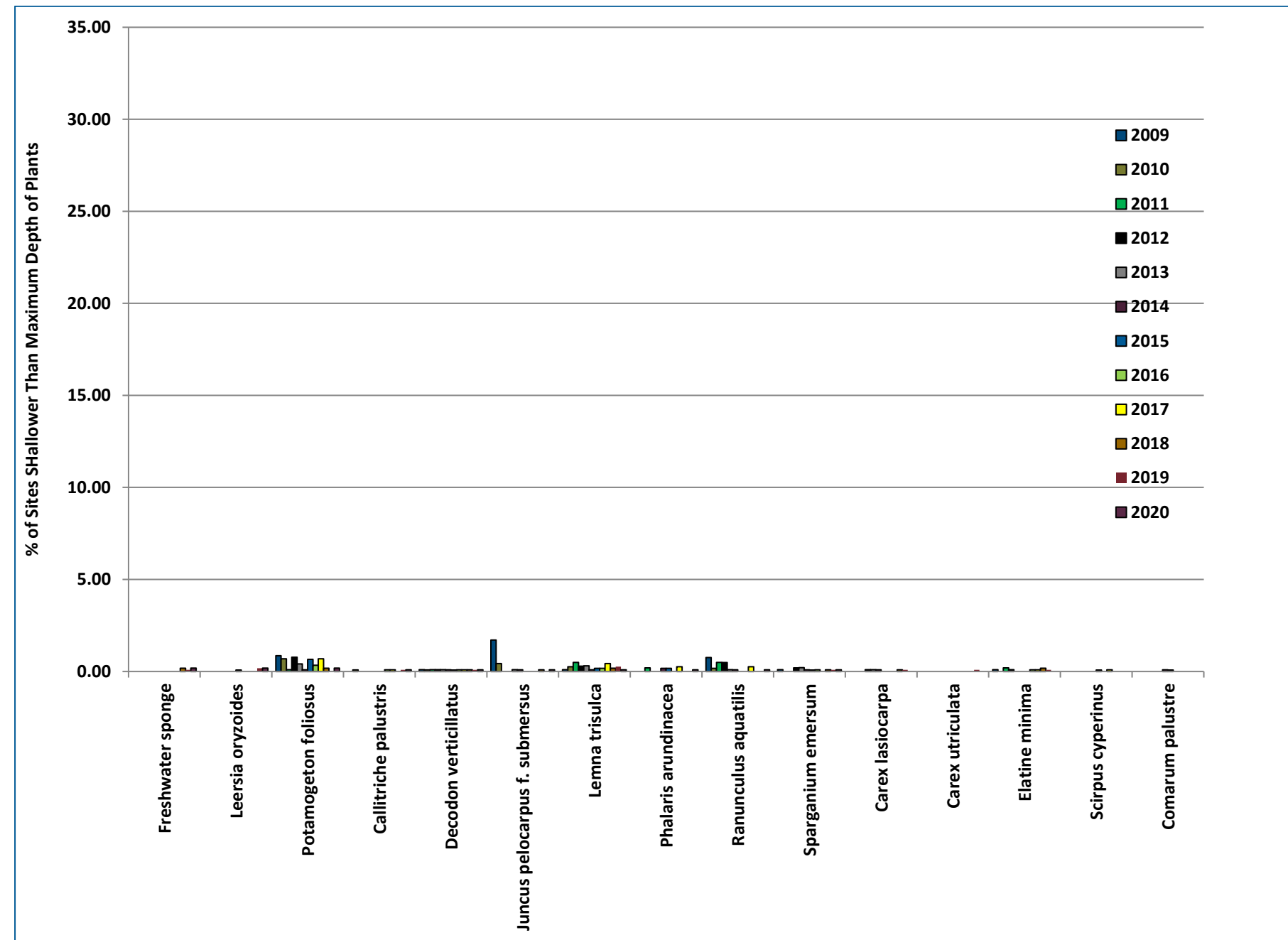
Figure 8-5 2009-2020 Beaver Dam Lake Frequency of Occurrence (% of Sites Shallower Than Maximum Depth of Plants)
