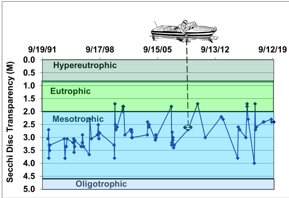
Figure 5-5 1992-2019 Beaver Dam Lake Secchi Disc Transparencies: Library Lake
