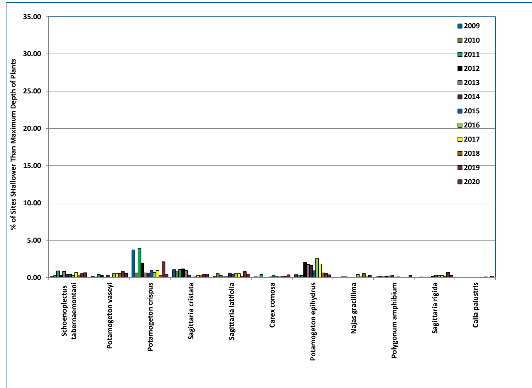
Figure 8-4 2009-2020 Beaver Dam Lake Frequency of Occurrence (% of Sites Shallower Than Maximum Depth of Plants)
