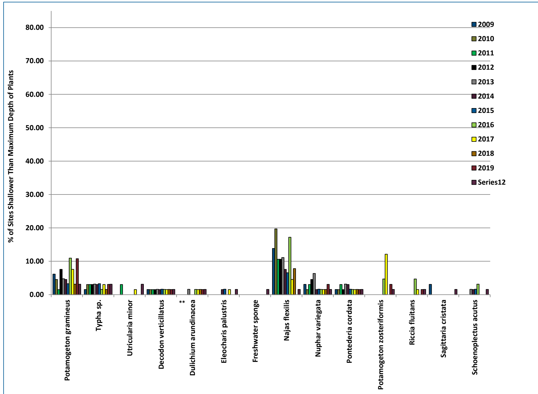
Figure 8-29 2009-2020 Norwegian Bay Frequency of Occurrence (% of Sites Shallower Than Maximum Depth of Plants)
