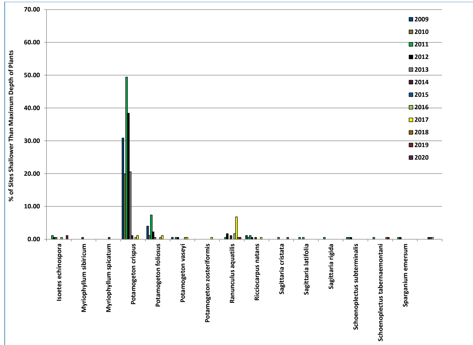
Figure 8-25 2009-2020 City Bay Frequency of Occurrence (% of Sites Shallower Than Maximum Depth of Plants)
