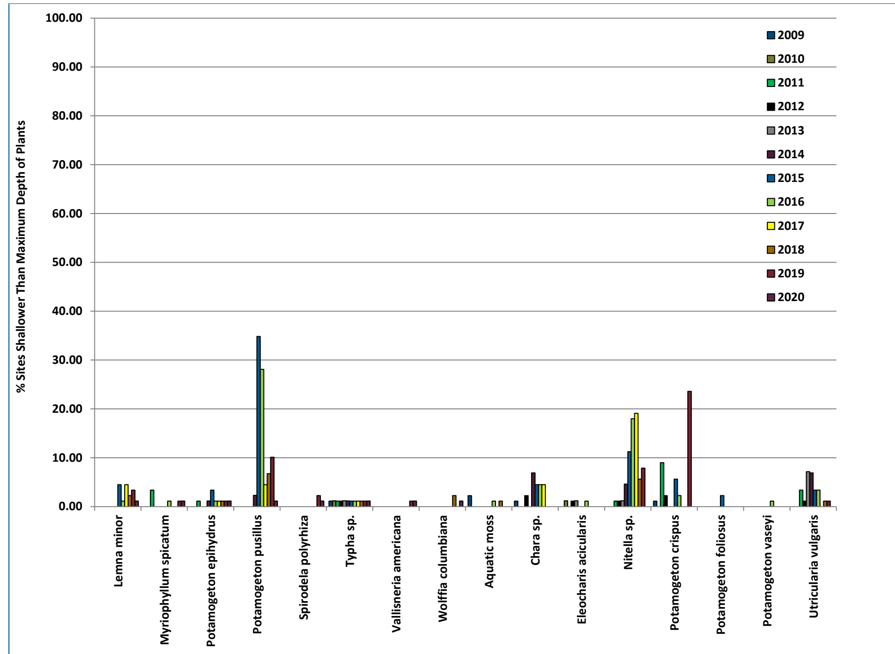
Figure 8-22 2009-2020 Cemetery Bay Frequency of Occurrence (% of Sites Shallower Than Maximum Depth of Plants)
