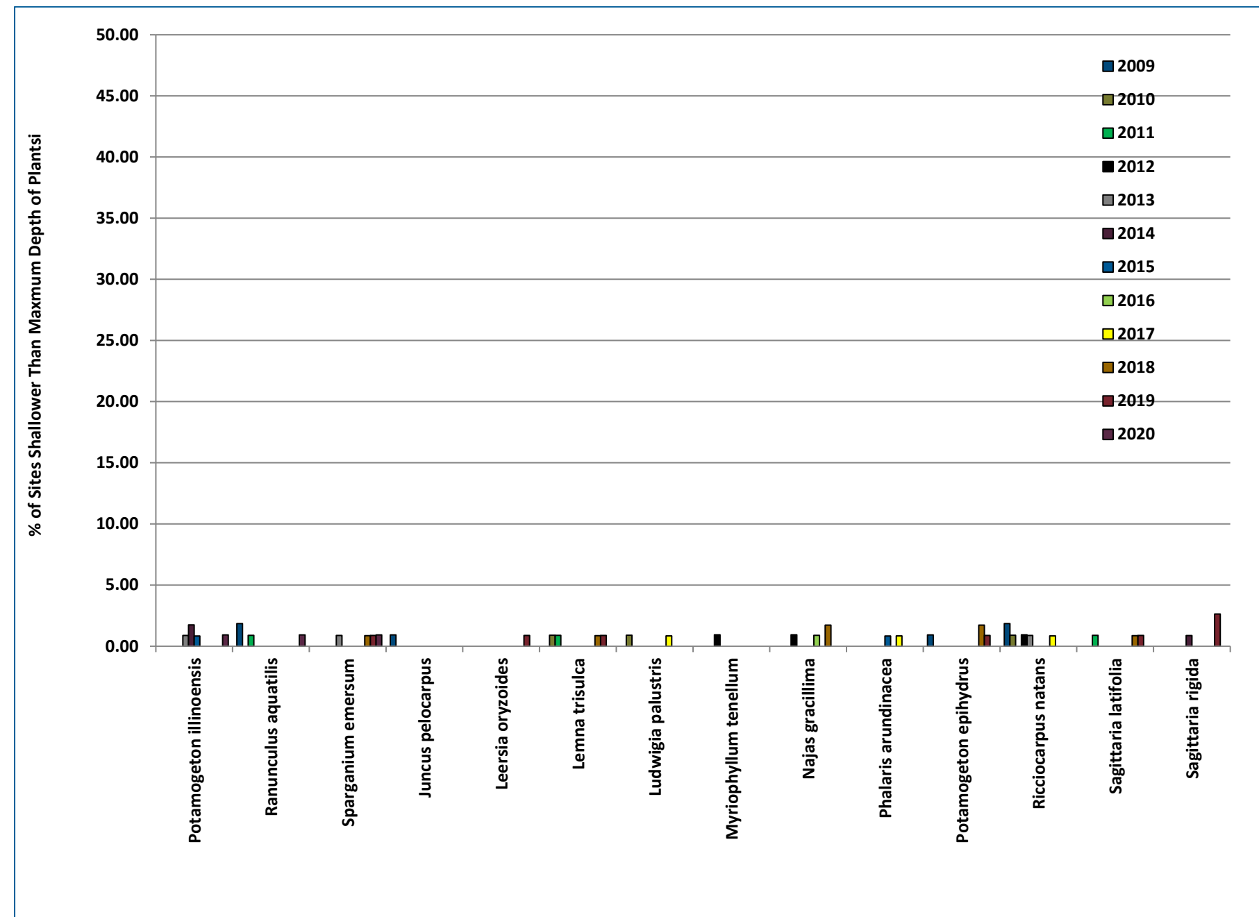
Figure 8-16 2009-2020 Rabbit Island Bay Frequency of Occurrence (% of Sites Shallower Than Maximum Depth of Plants)
