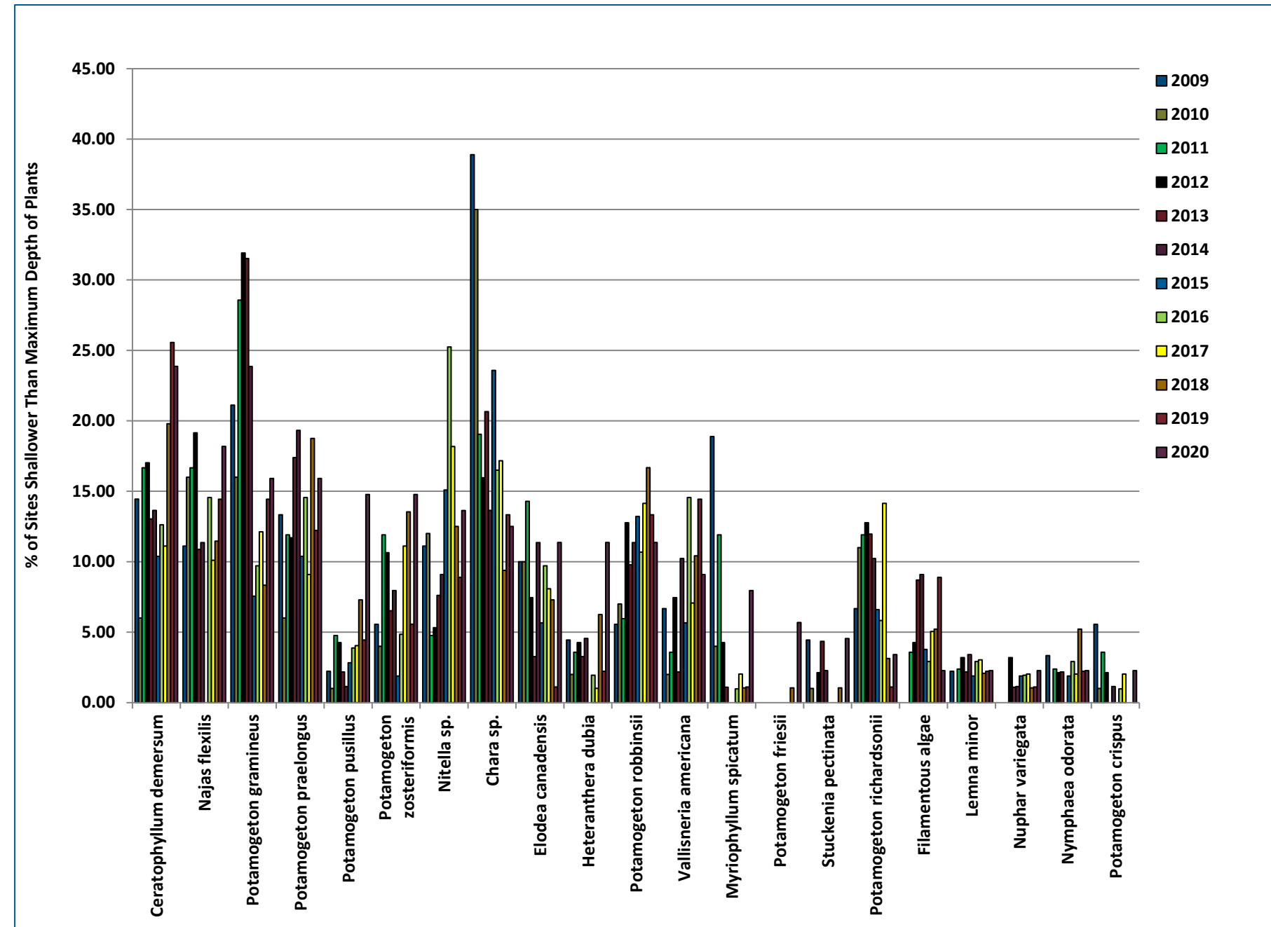
Figure 8-11 2009-2020 Williams Bay Frequency of Occurrence (% of Sites Shallower Than Maximum Depth of Plants)
