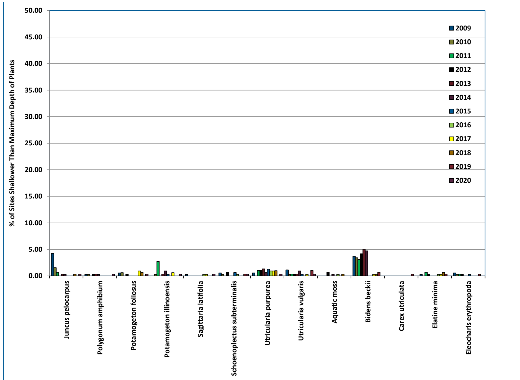
Figure 8-9 2009-2020 West Lake Frequency of Occurrence (% of Sites Shallower Than Maximum Depth of Plants)
