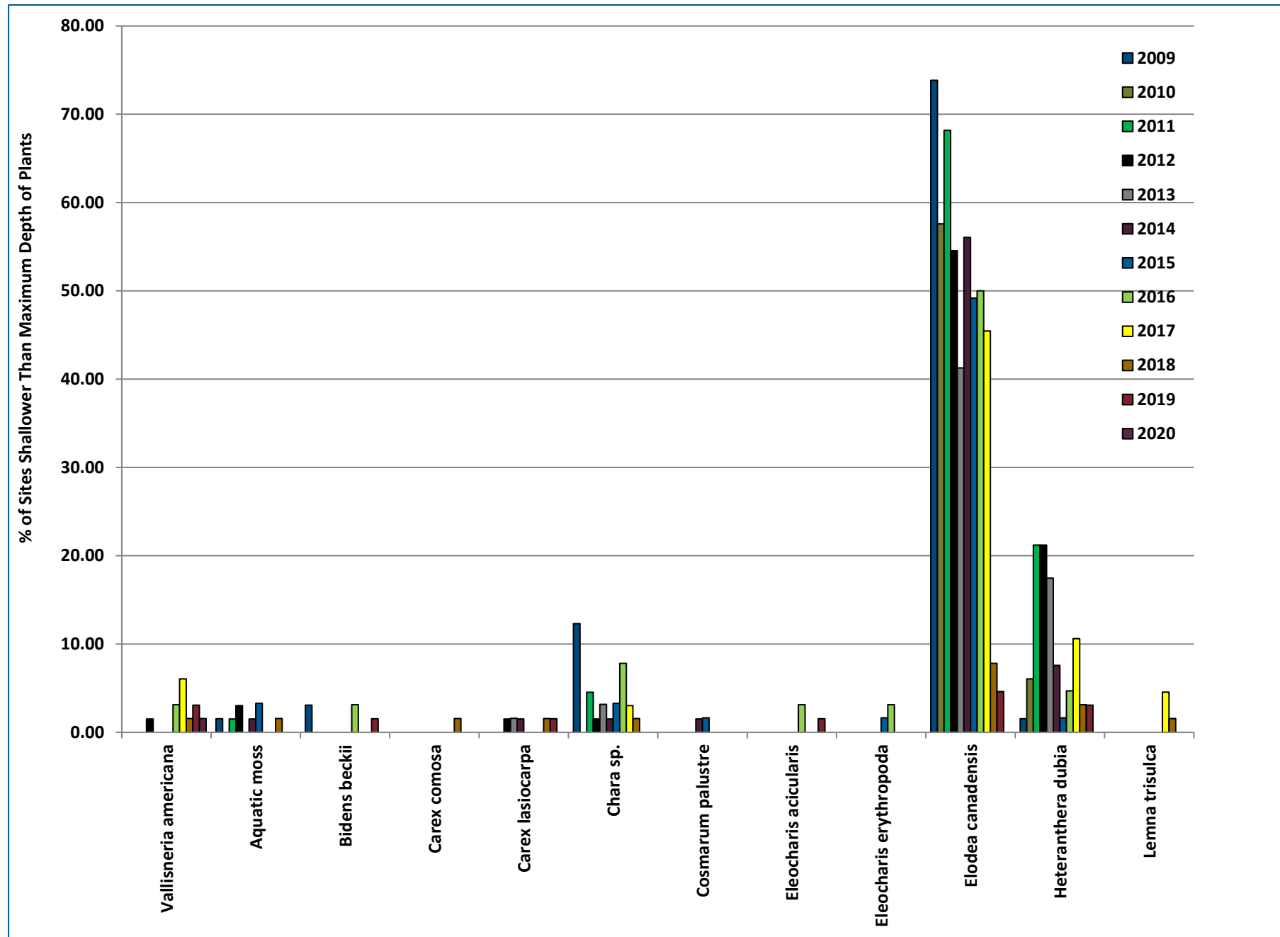
Figure 8-30 2009-2020 Norwegian Bay Frequency of Occurrence (% of Sites Shallower Than Maximum Depth of Plants)
