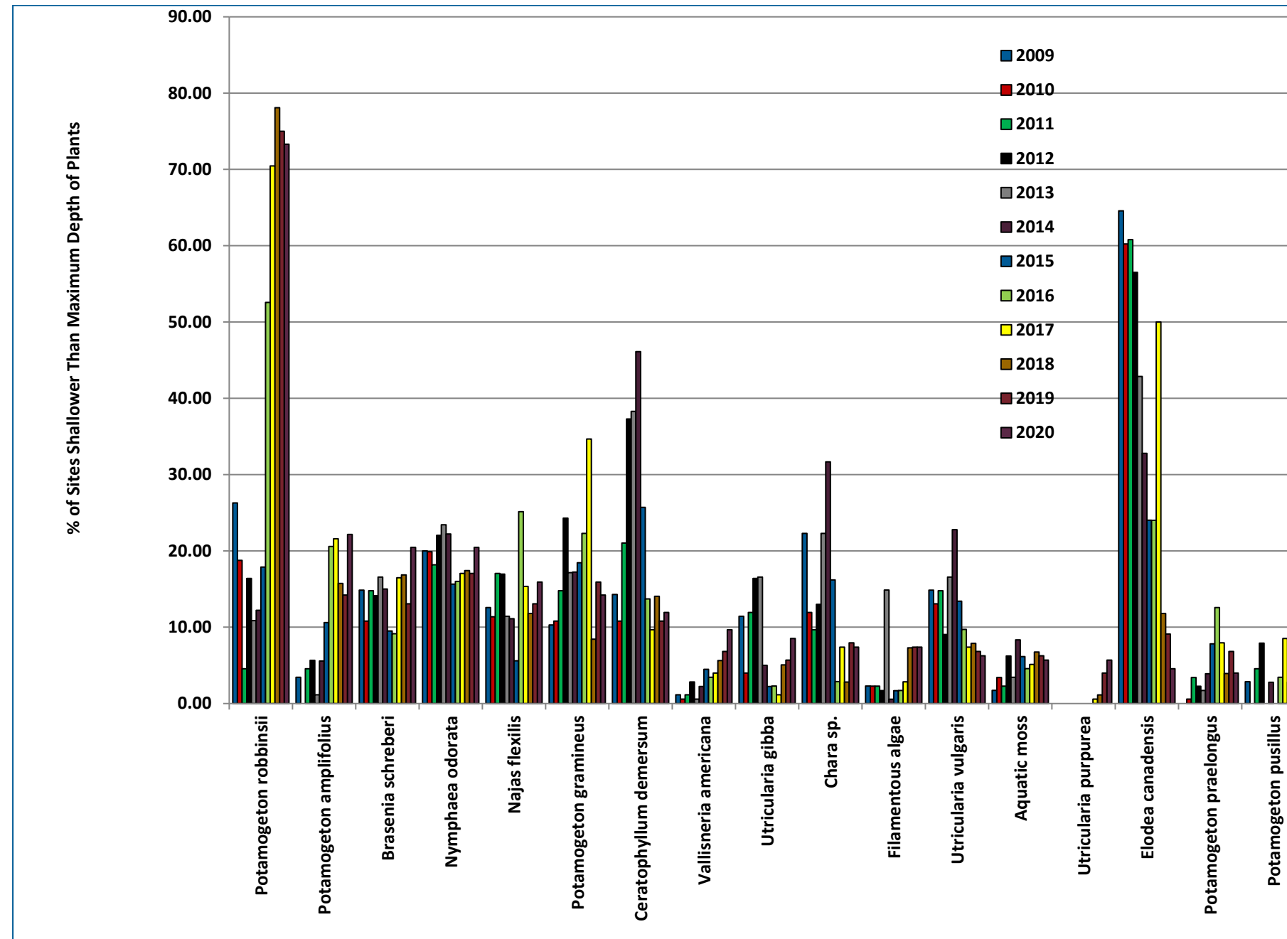
Figure 8-23 2009-2020 City Bay Frequency of Occurrence (% of Sites Shallower Than Maximum Depth of Plants)
