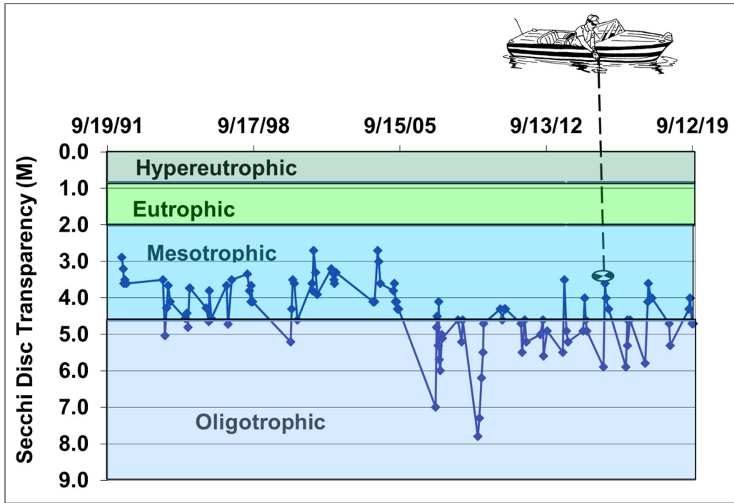
Figure 5-3 1992-2019 Beaver Dam Lake Secchi Disc Transparencies: Williams Bay
