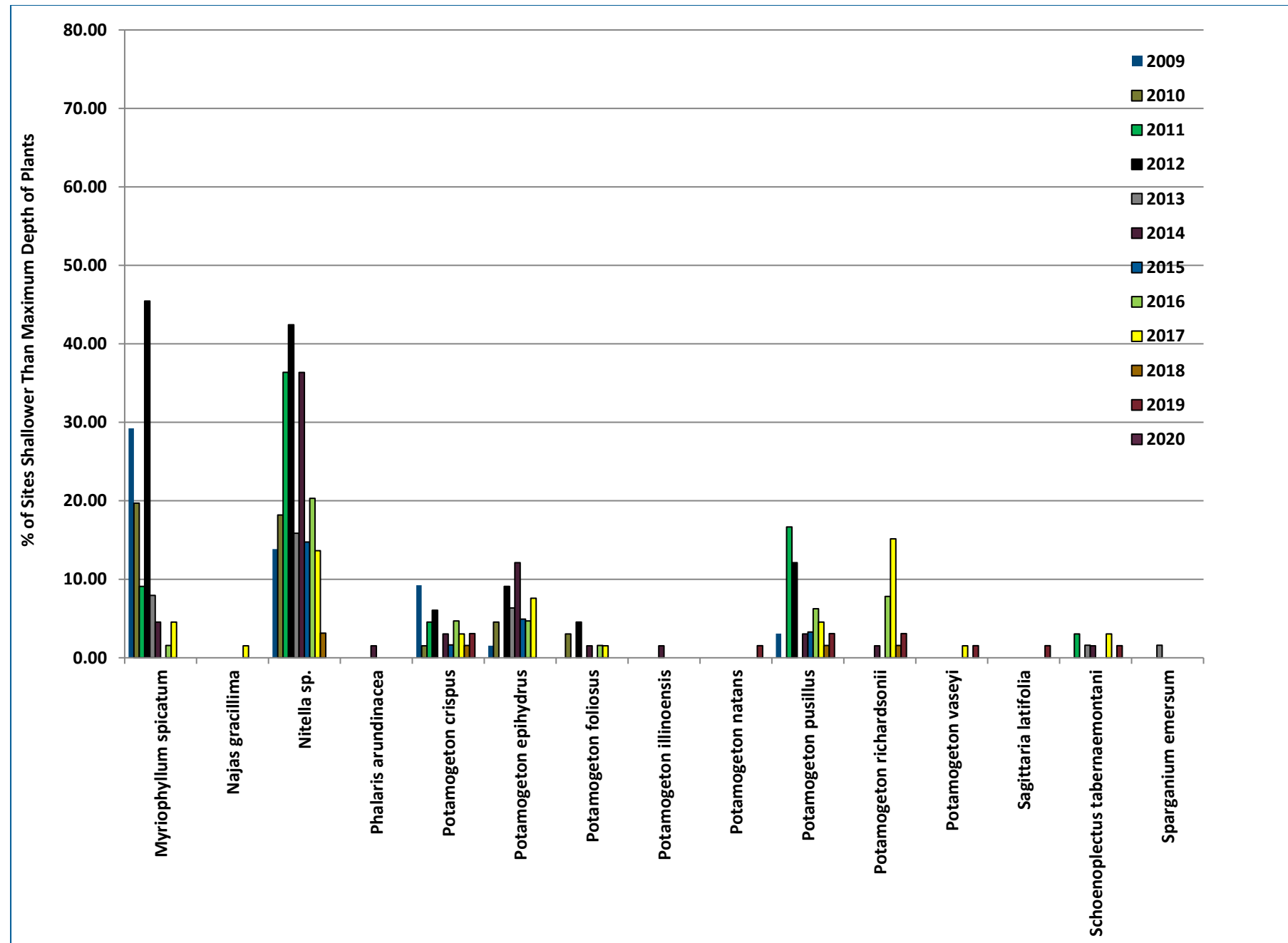
Figure 8-31 2009-2020 Norwegian Bay Frequency of Occurrence (% of Sites Shallower Than Maximum Depth of Plants)
