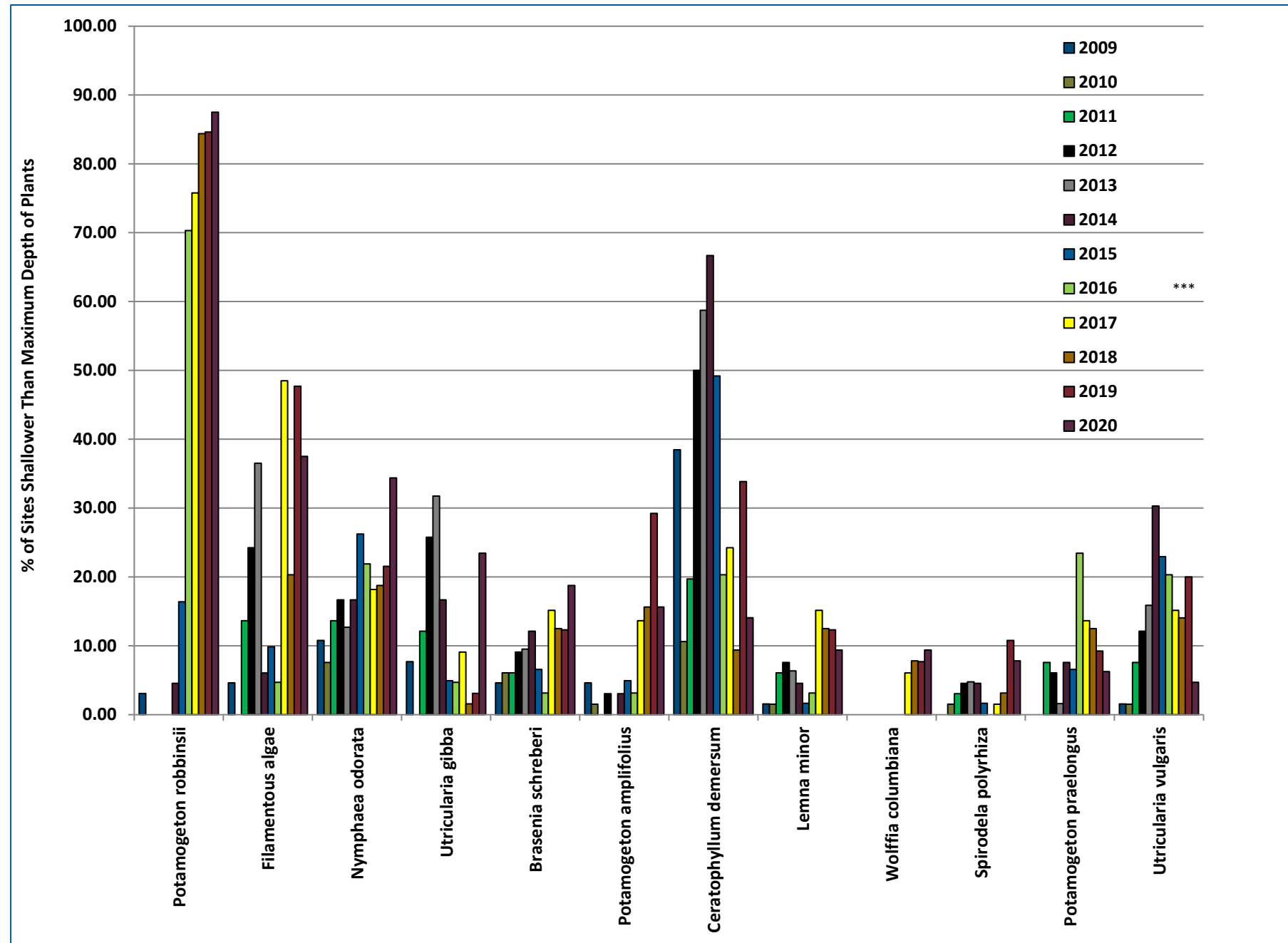
Figure 8-28 2009-2020 Norwegian Bay Frequency of Occurrence (% of Sites Shallower Than Maximum Depth of Plants)
