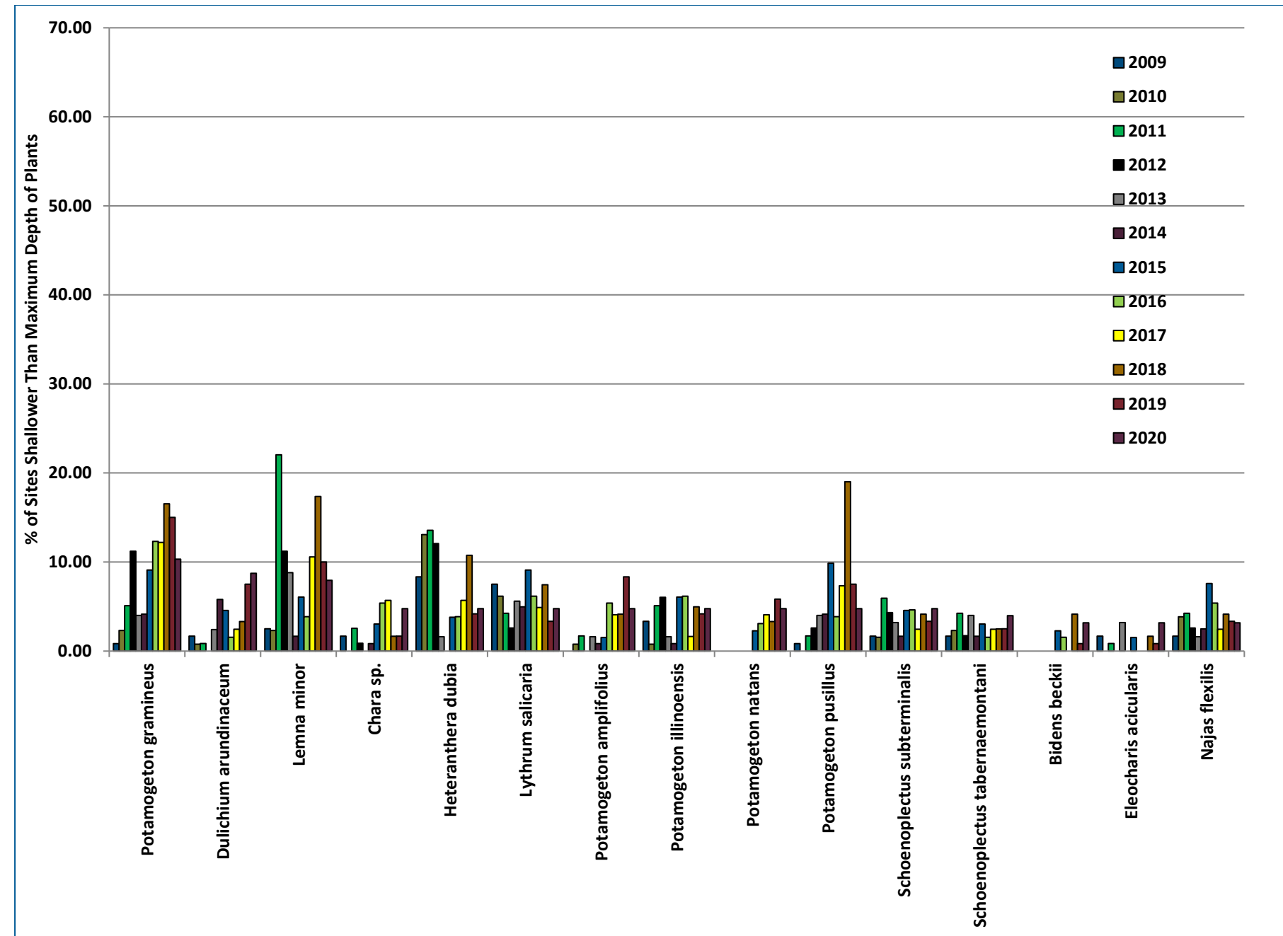
Figure 8-18 2009-2020 Library Lake Frequency of Occurrence (% of Sites Shallower Than Maximum Depth of Plants)
