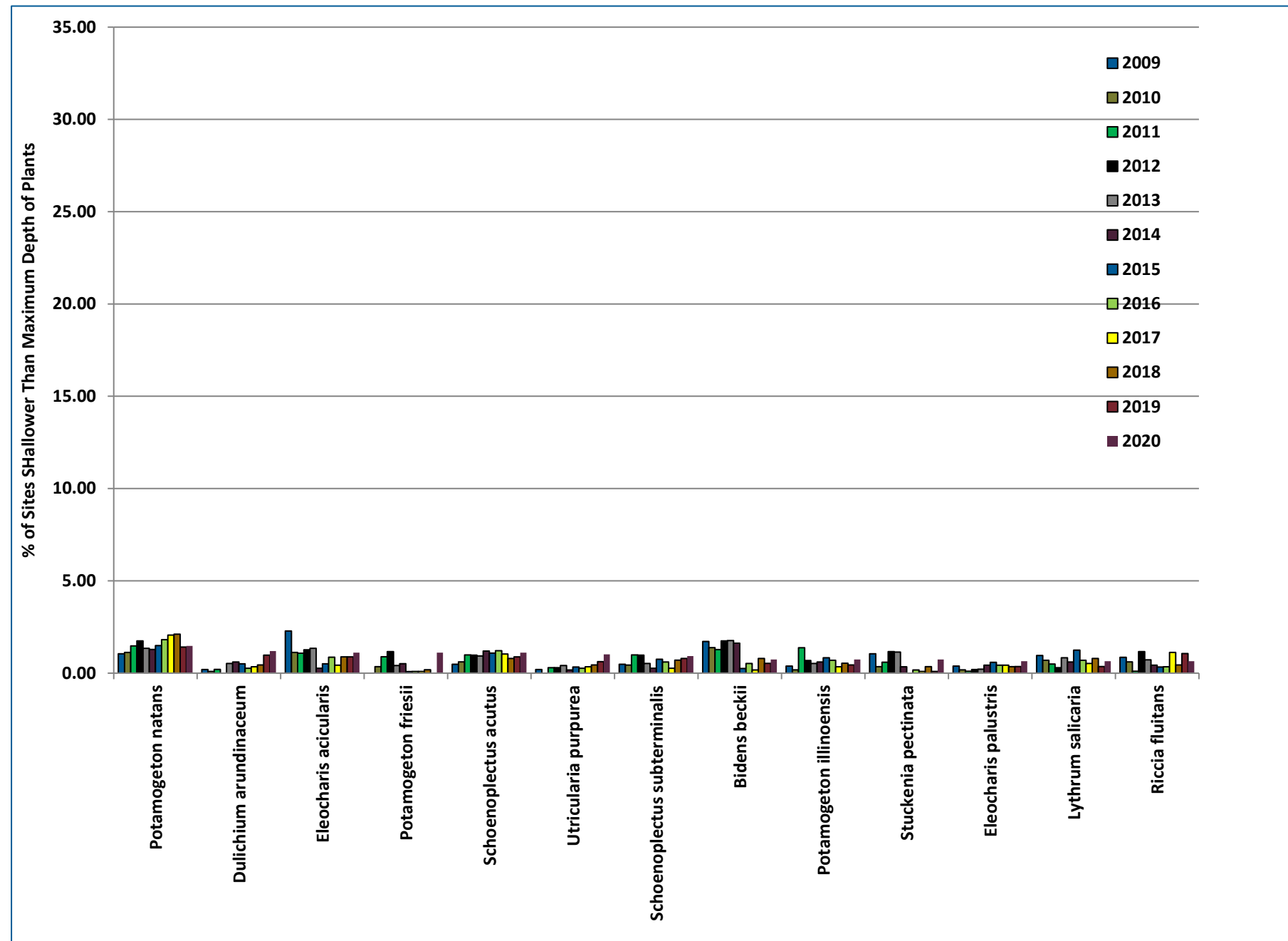
Figure 8-3 2009-2020 Beaver Dam Lake Frequency of Occurrence (% of Sites Shallower Than Maximum Depth of Plants)
