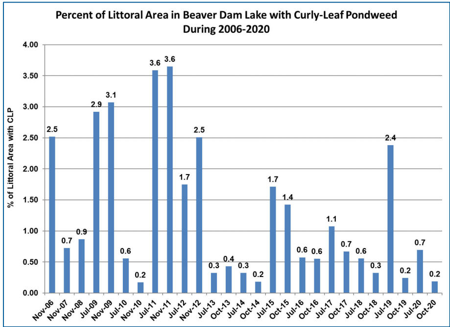
Figure 7-4 Percent of Littoral Area of Beaver Dam Lake with Curly-leaf Pondweed during 2006-2020
