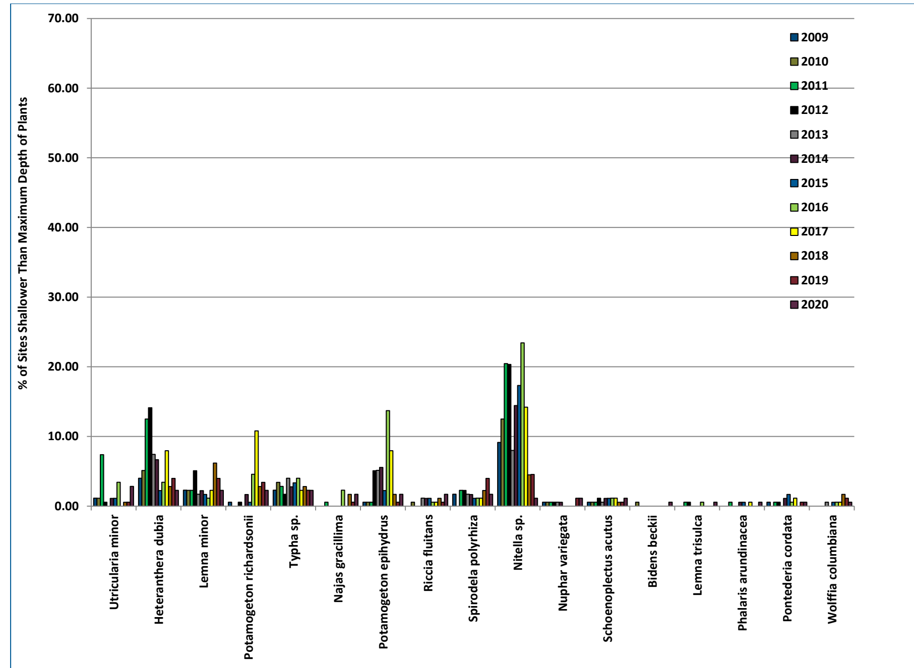
Figure 8-24 2009-2020 City Bay Frequency of Occurrence (% of Sites Shallower Than Maximum Depth of Plants)
