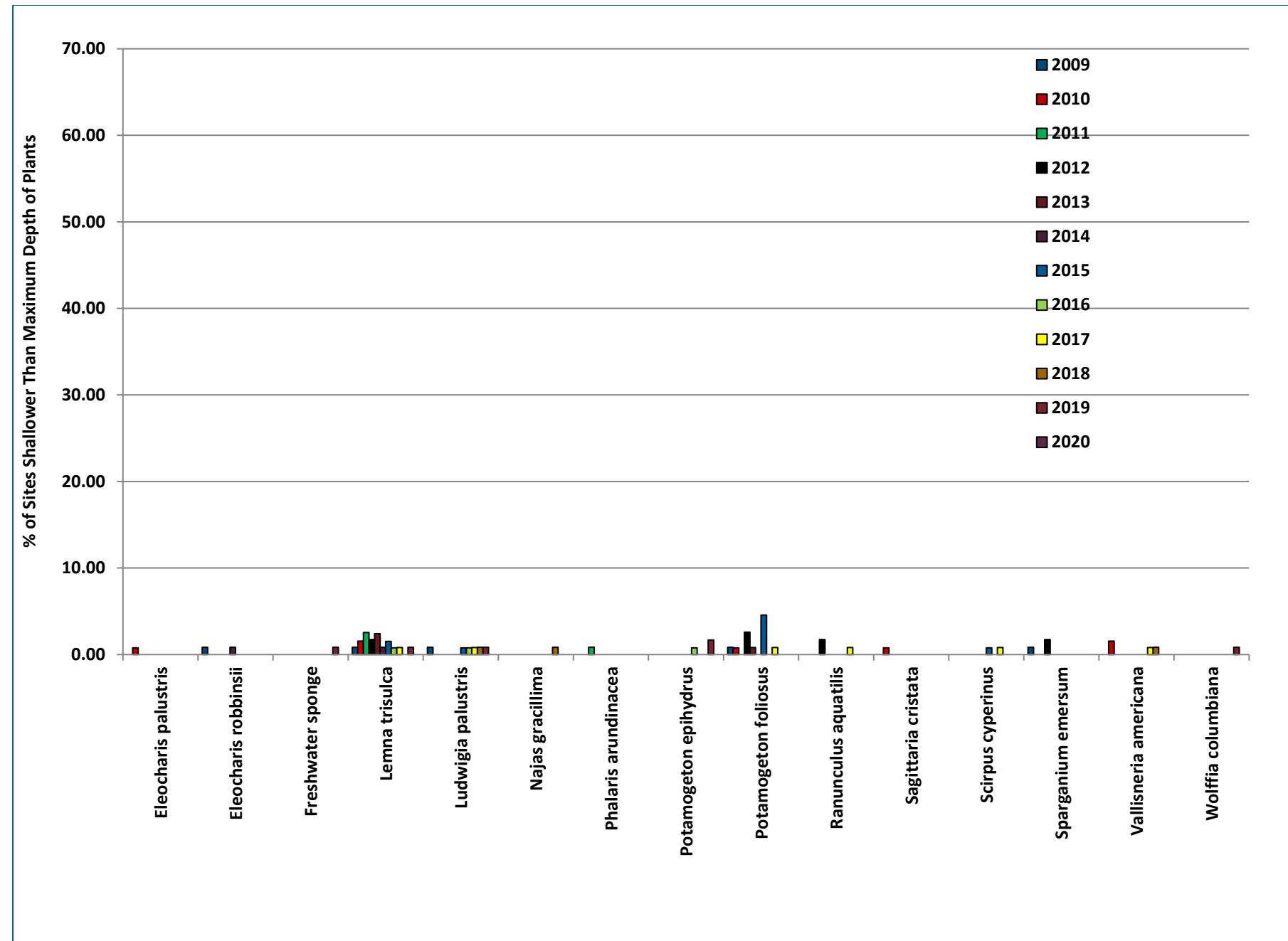
Figure 8-20 2009-2020 Library Lake Frequency of Occurrence (% of Sites Shallower Than Maximum Depth of Plants)
