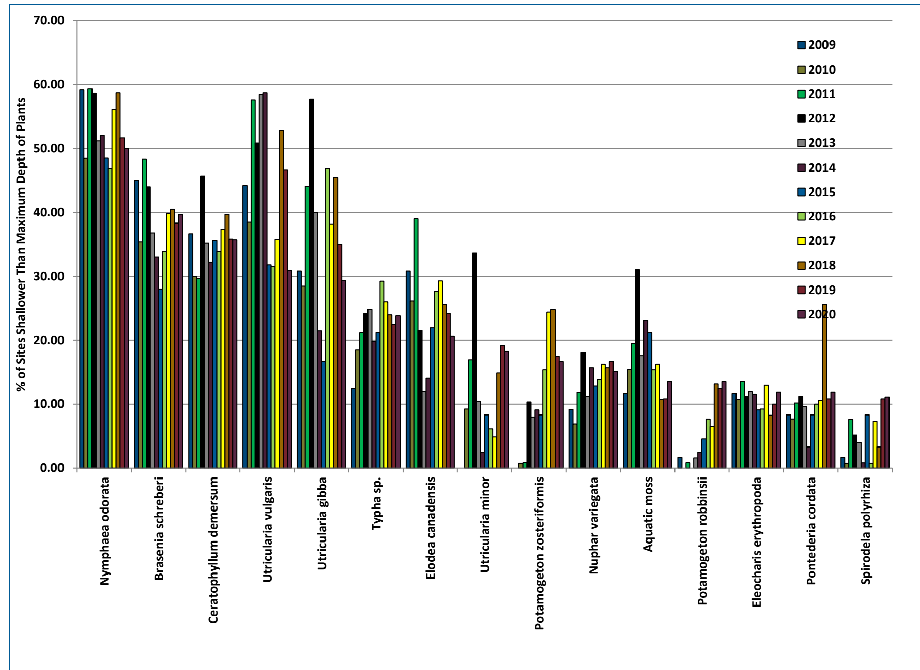
Figure 8-17 2009-2020 Library Lake Frequency of Occurrence (% of Sites Shallower Than Maximum Depth of Plants)
