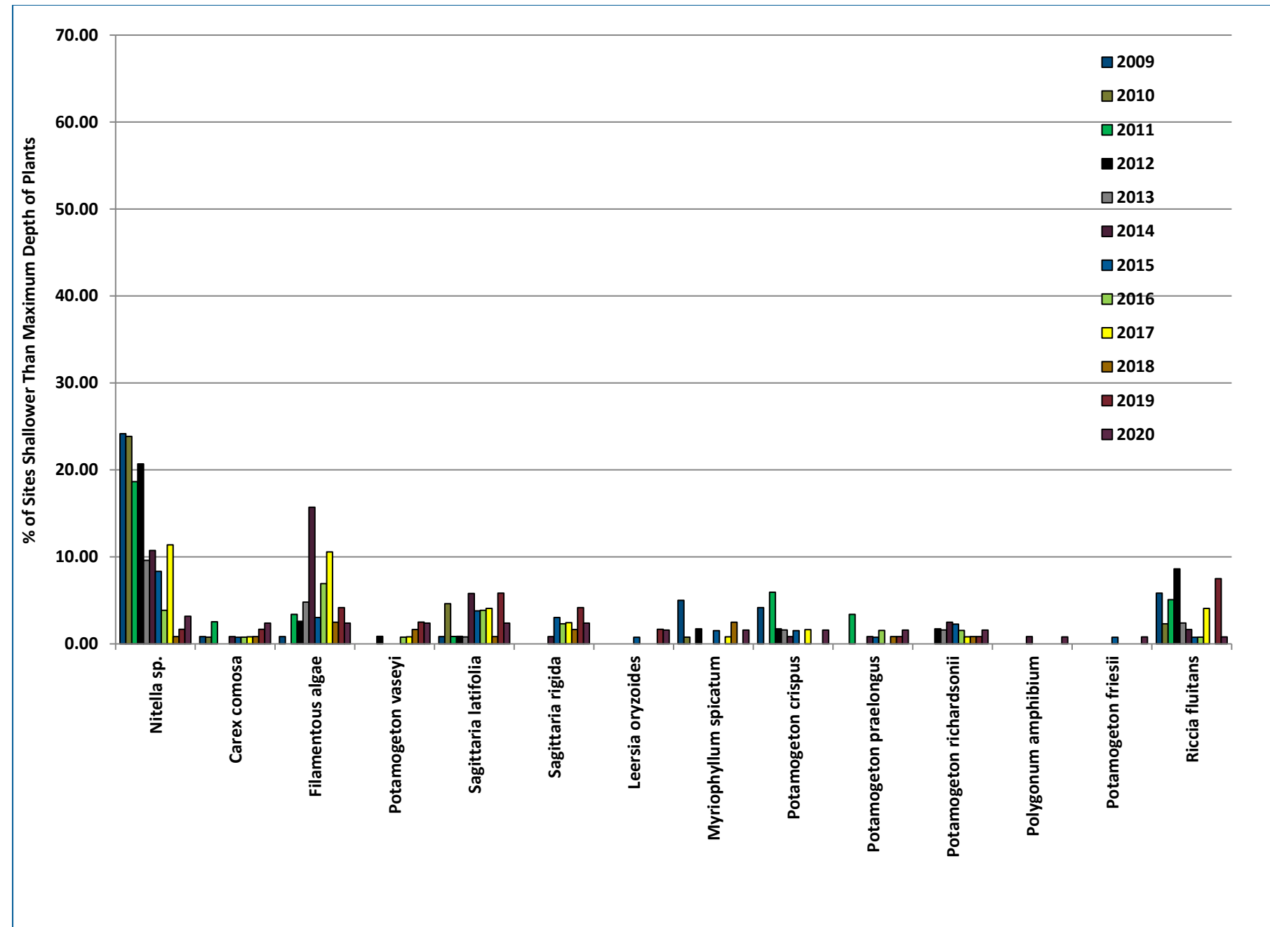
Figure 8-19 2009-2020 Library Lake Frequency of Occurrence (% of Sites Shallower Than Maximum Depth of Plants)
