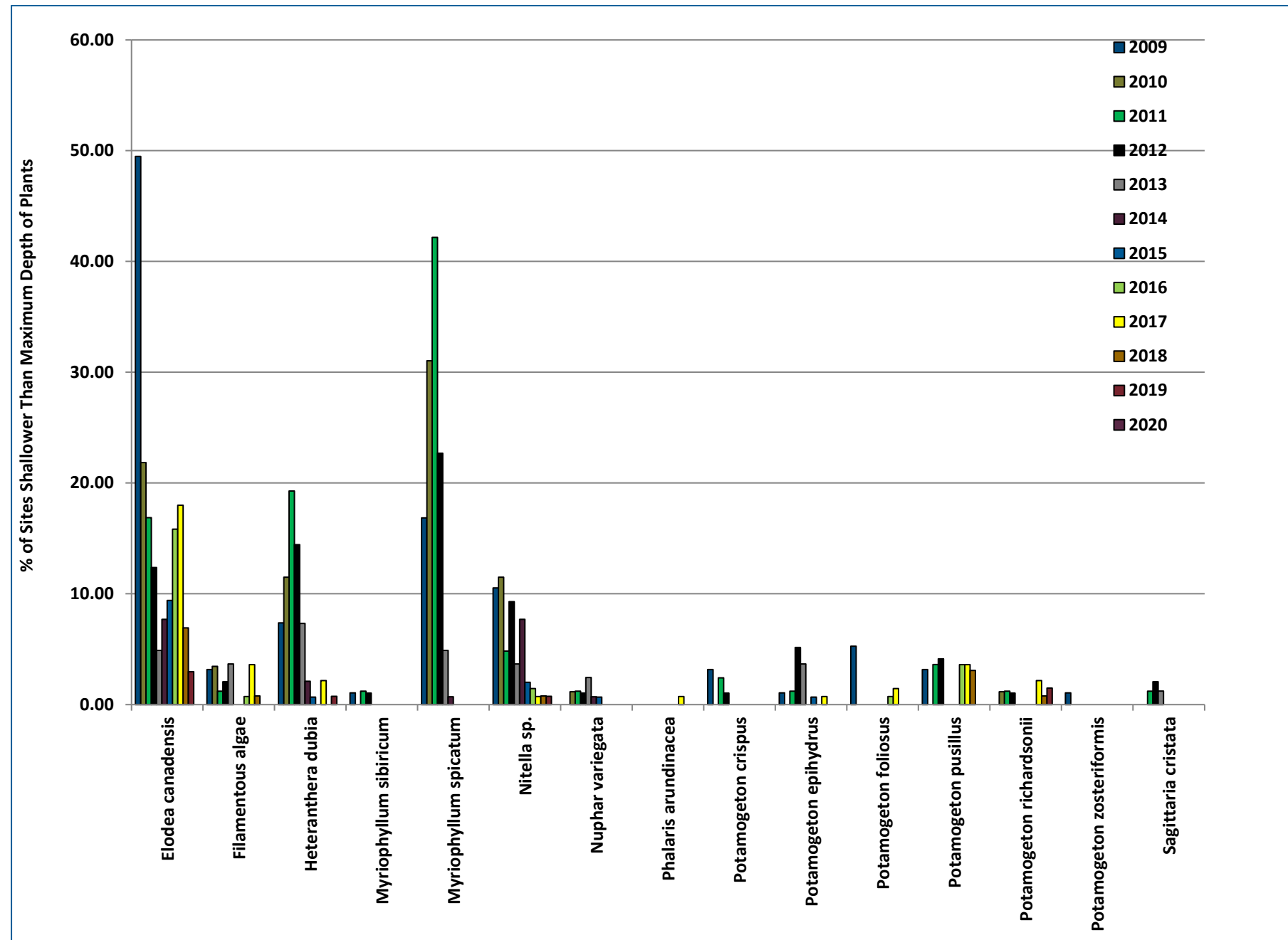
Figure 8-27 2009-2020 East Lake Frequency of Occurrence (% of Sites Shallower Than Maximum Depth of Plants)
