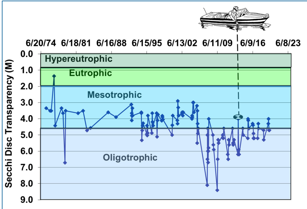
Figure 5-1 1975-2019 Beaver Dam Lake Secchi Disc Transparencies: West Lake (West End)
