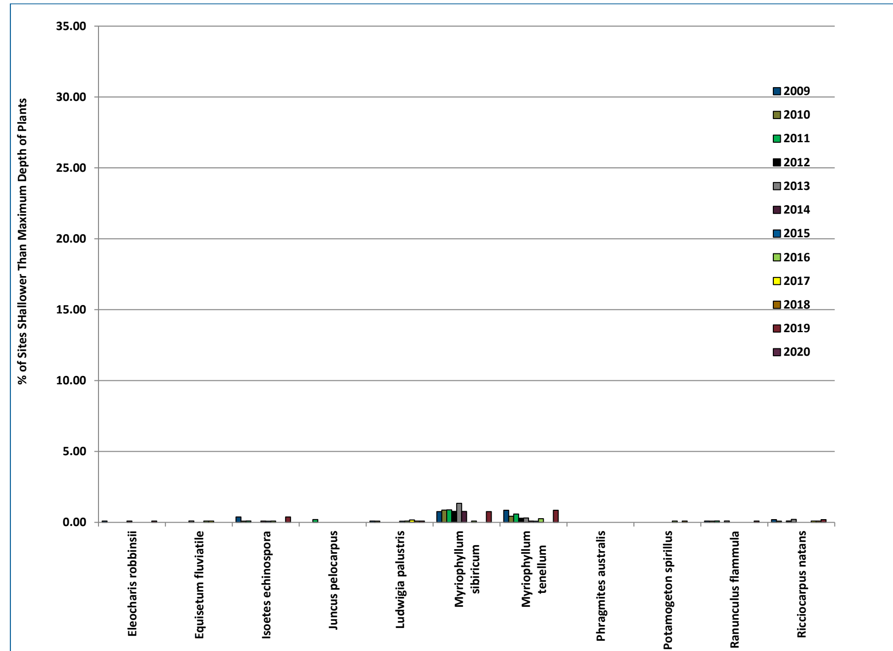
Figure 8-6 2009-2020 Beaver Dam Lake Frequency of Occurrence (% of Sites Shallower Than Maximum Depth of Plants)
