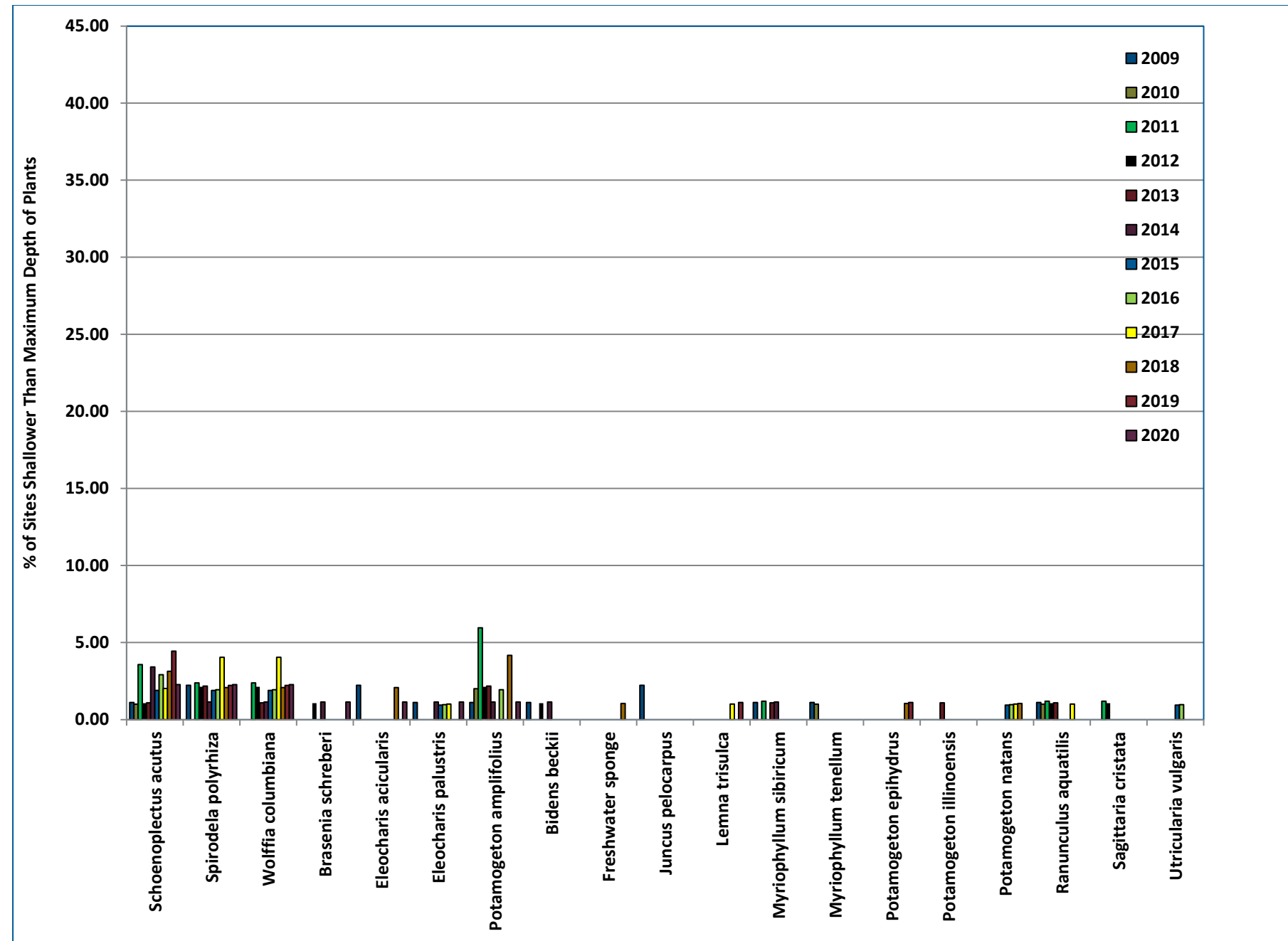
Figure 8-12 2009-2020 Williams Bay Lake Frequency of Occurrence (% of Sites Shallower Than Maximum Depth of Plants)
