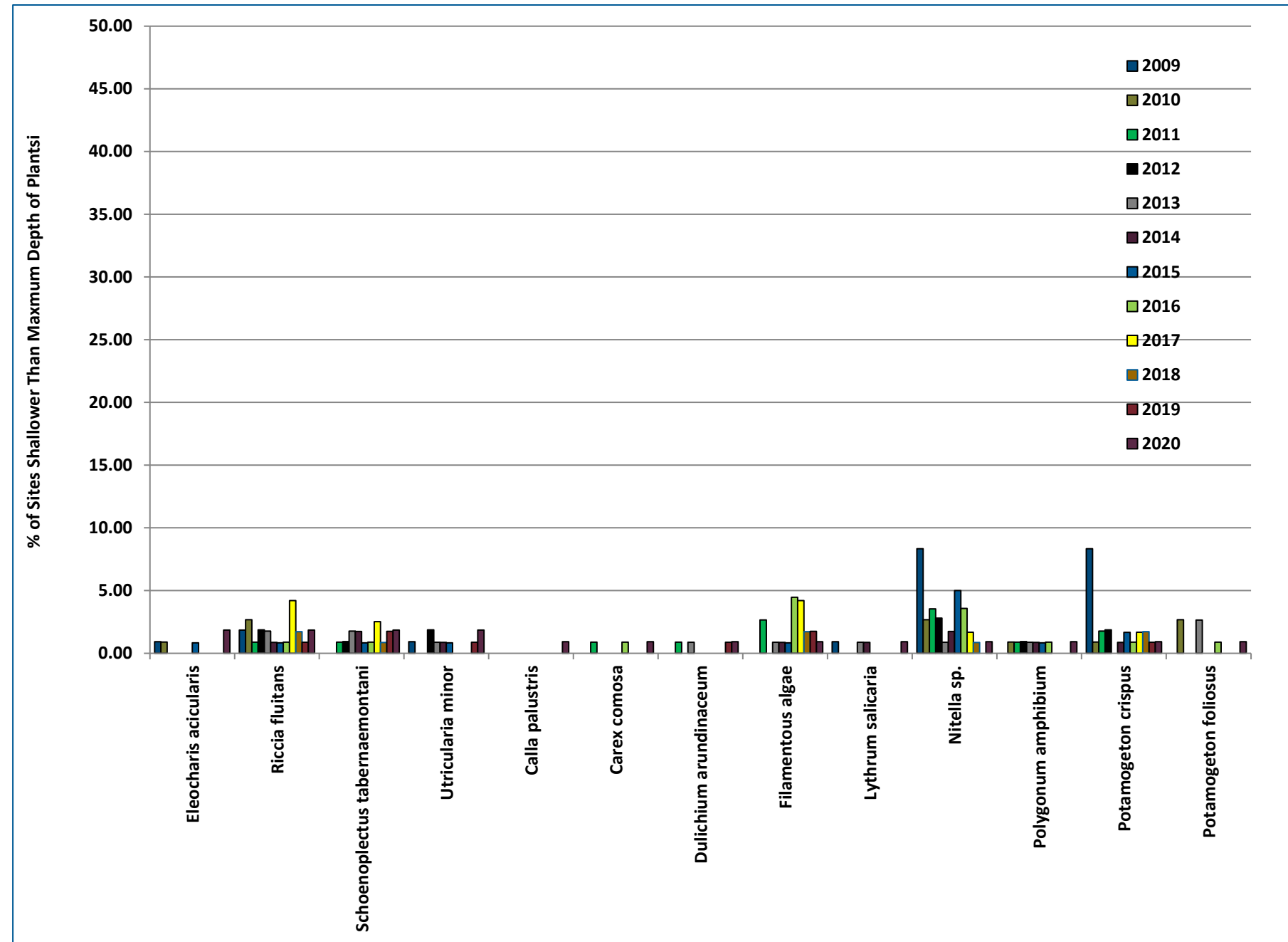
Figure 8-15 2009-2020 Rabbit Island Bay Frequency of Occurrence (% of Sites Shallower Than Maximum Depth of Plants)
