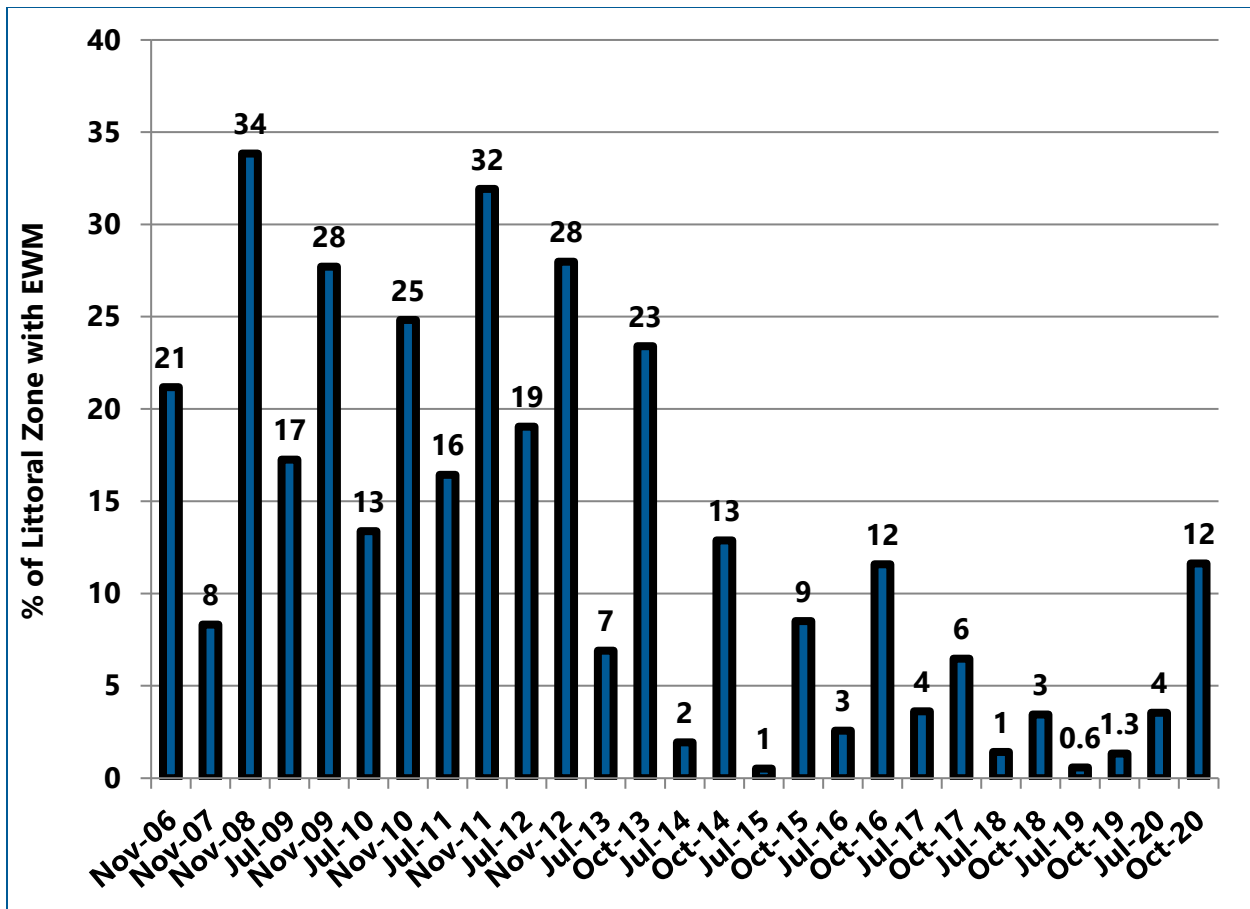
Figure 7-5 Percent of Littoral Area of Beaver Dam Lake with EWM during 2006-2020
