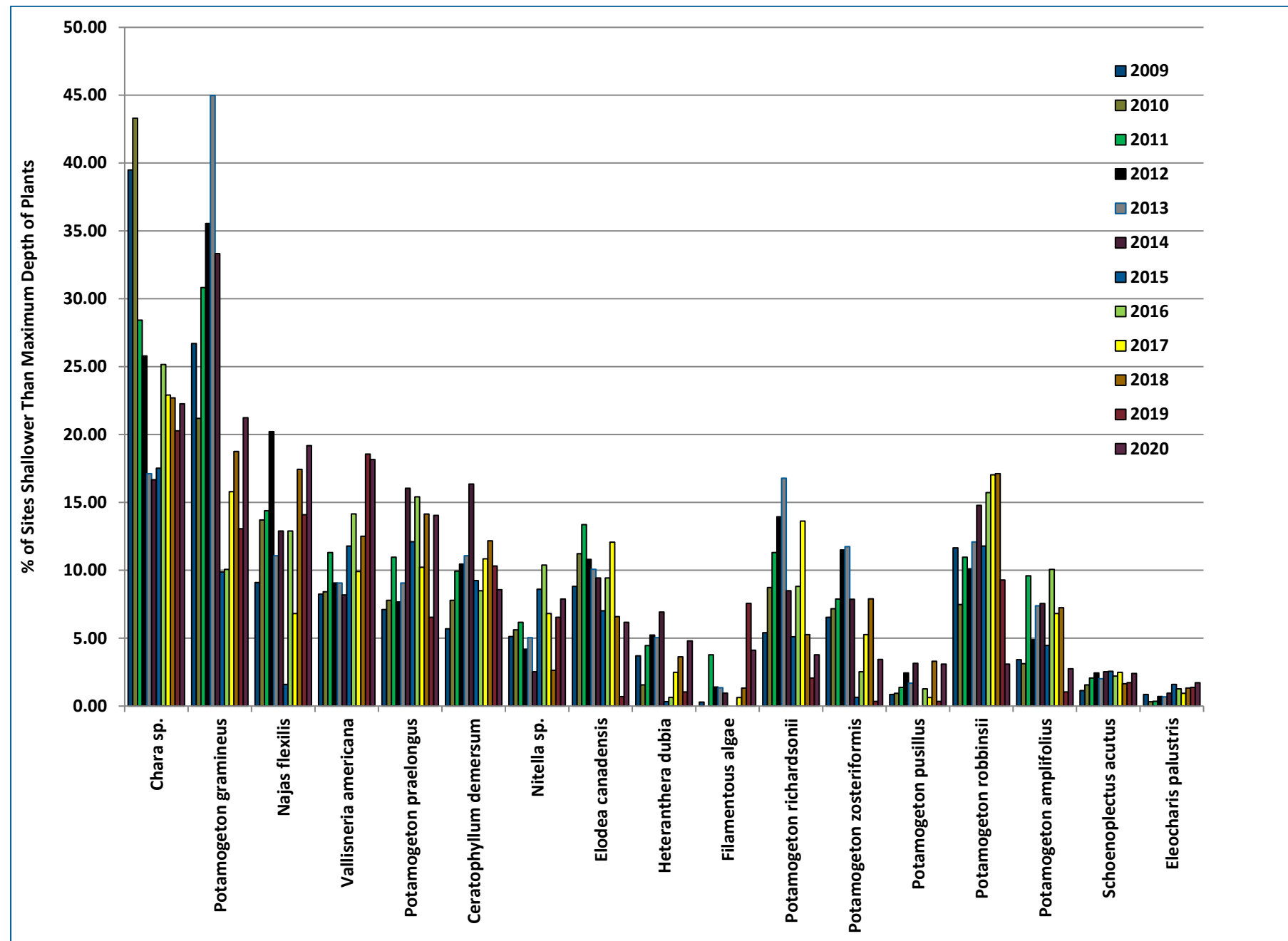
Figure 8-7 2009-2020 West Lake Frequency of Occurrence (% of Sites Shallower Than Maximum Depth of Plants)
