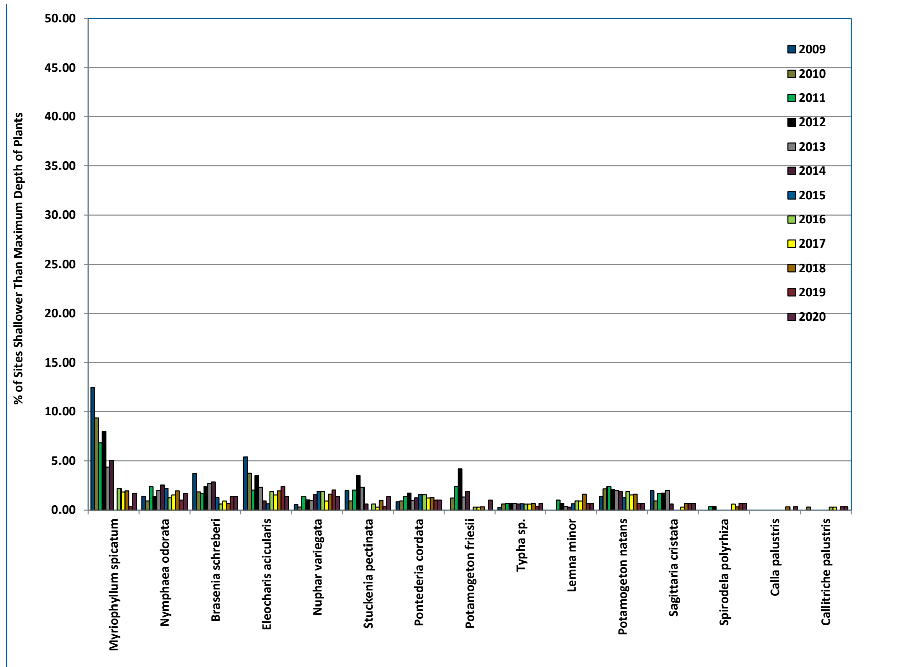
Figure 8-8 2009-2020 West Lake Frequency of Occurrence (% of Sites Shallower Than Maximum Depth of Plants)
