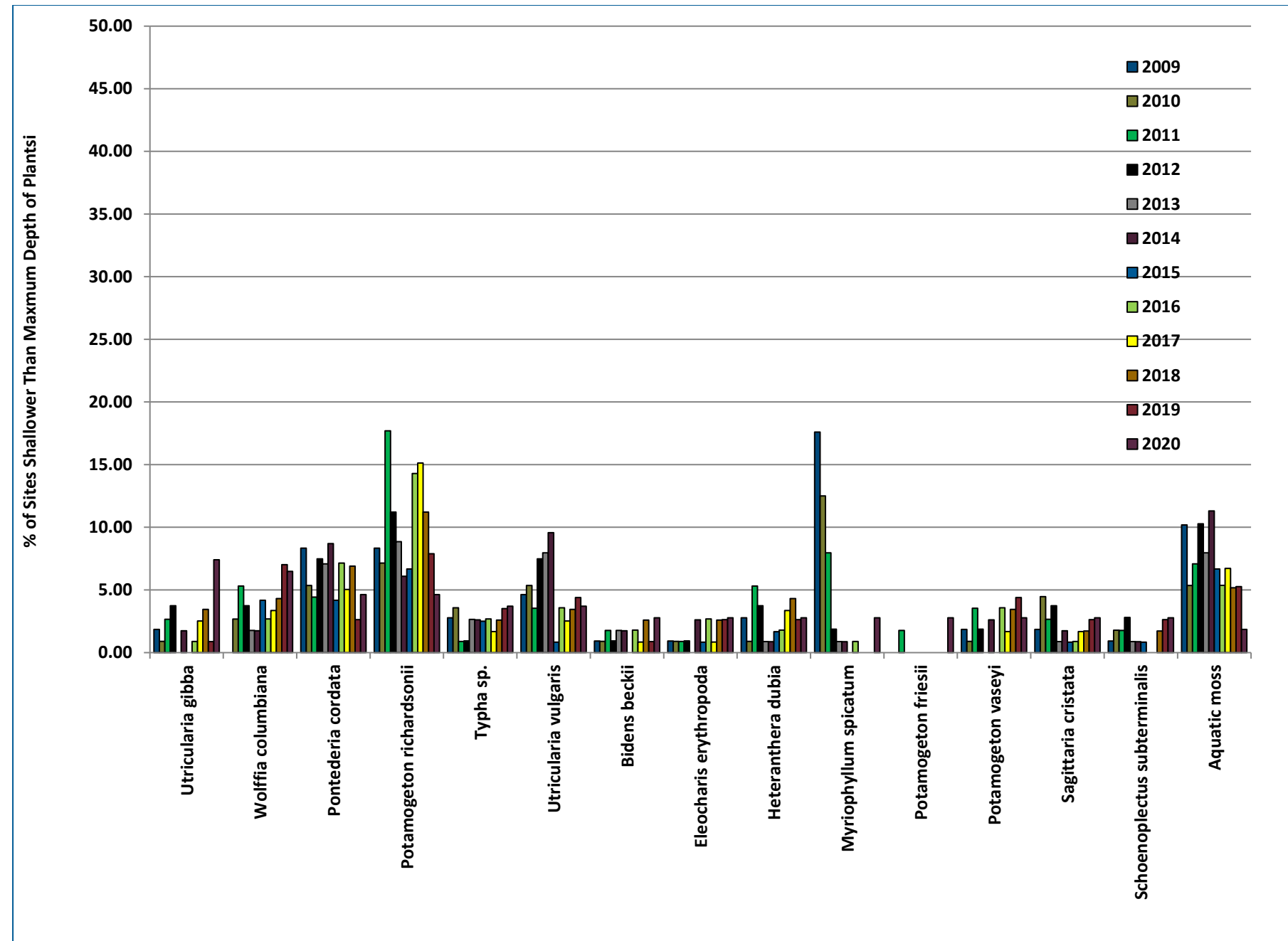
Figure 8-14 2009-2020 Rabbit Island Bay Frequency of Occurrence (% of Sites Shallower Than Maximum Depth of Plants)
