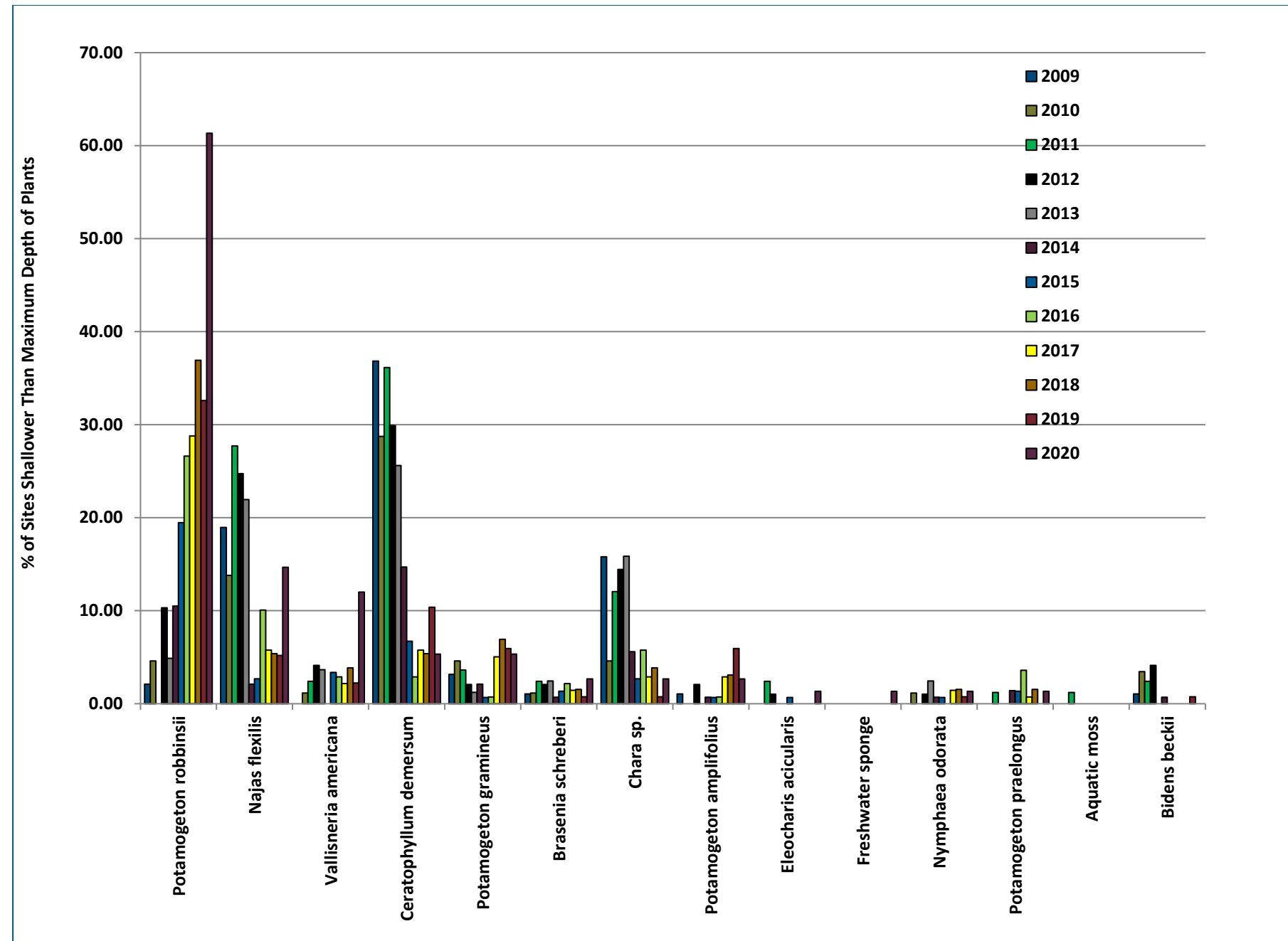
Figure 8-26 2009-2020 East Lake Frequency of Occurrence (% of Sites Shallower Than Maximum Depth of Plants)
