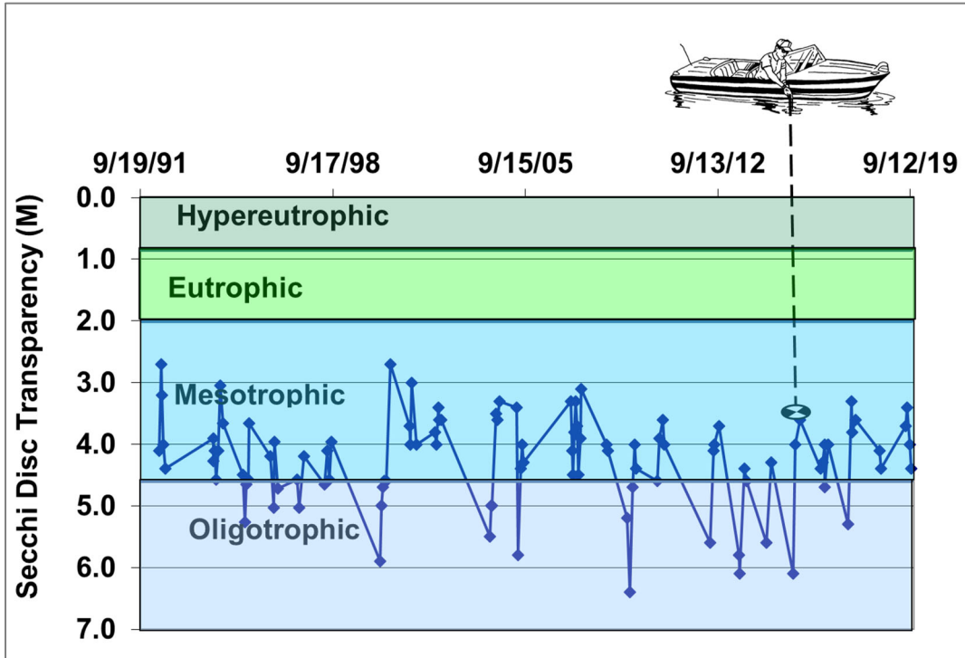
Figure 5-4 1992-2019 Beaver Dam Lake Secchi Disc Transparencies: Rabbit Island Bay
