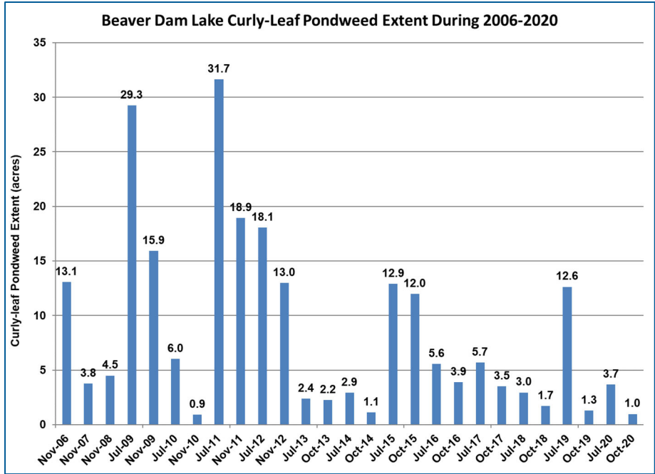
Figure 7-3 2006-2020 Beaver Dam Lake Curly-leaf Pondweed Extent
