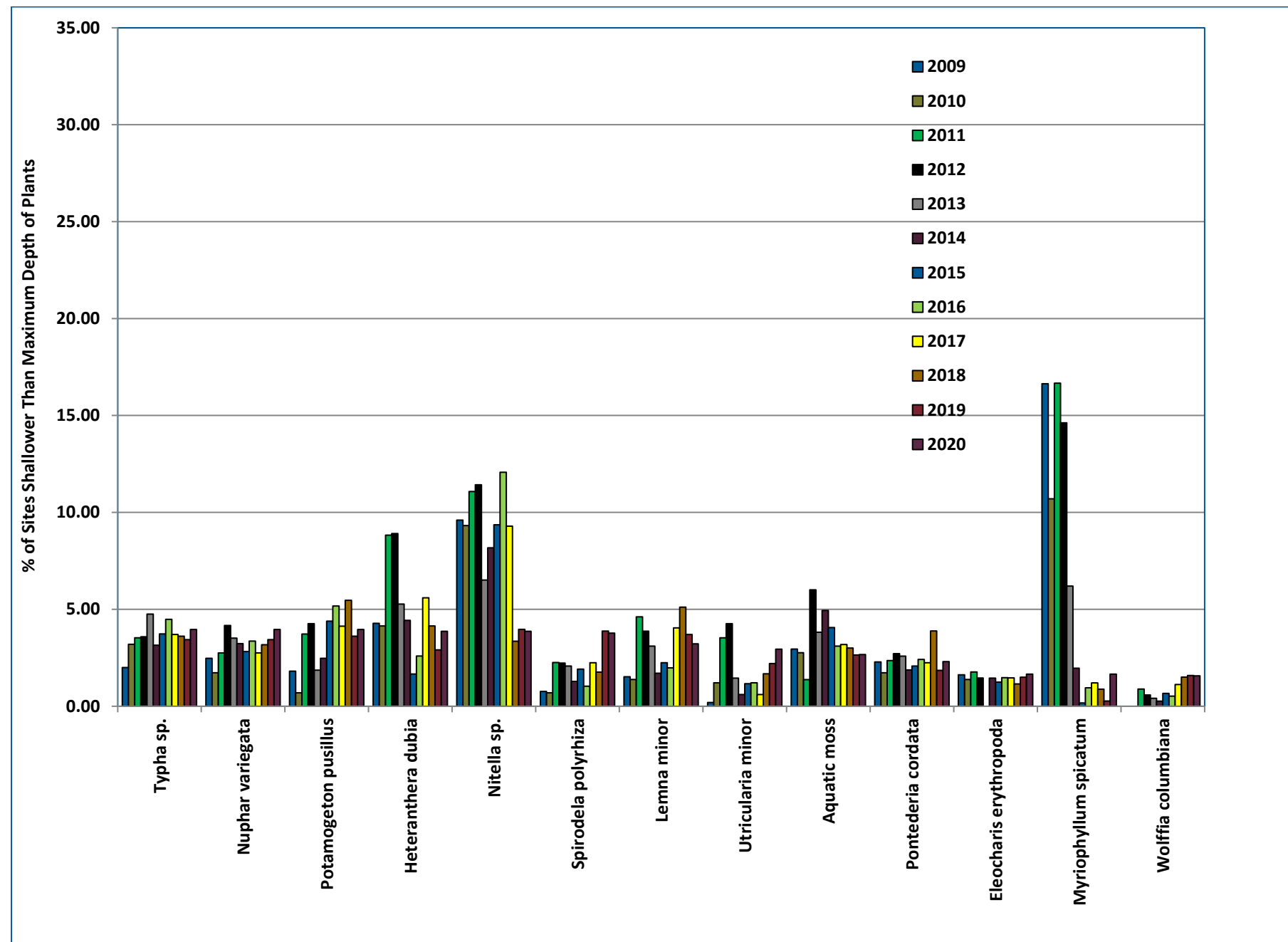
Figure 8-2 2009-2020 Beaver Dam Lake Frequency of Occurrence (% of Sites Shallower Than Maximum Depth of Plants)
