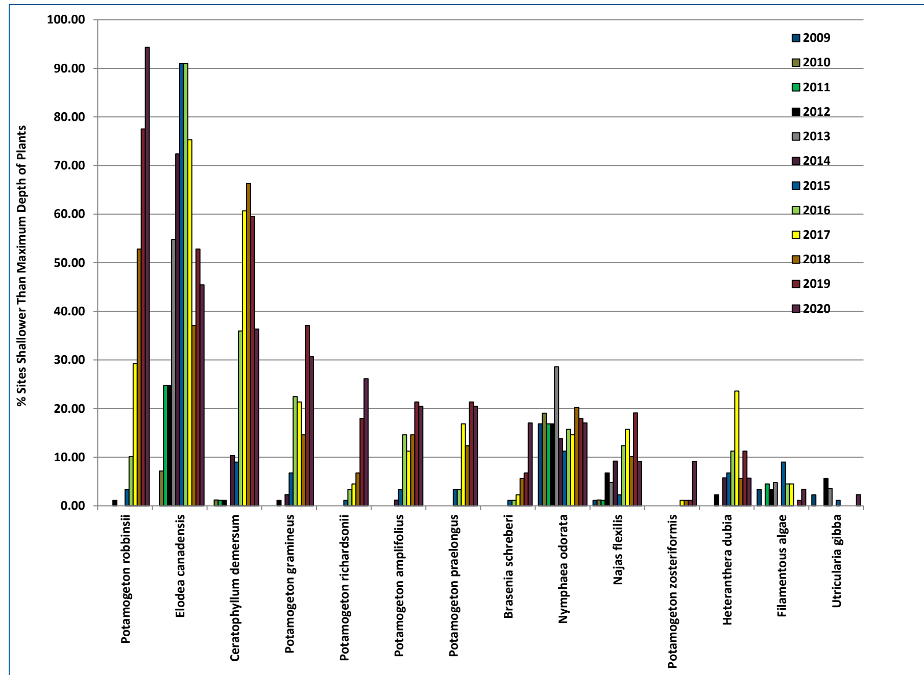
Figure 8-21 2009-2020 Cemetery Bay Frequency of Occurrence (% of Sites Shallower Than Maximum Depth of Plants)
